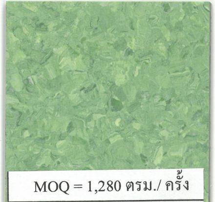
2605 Clark
