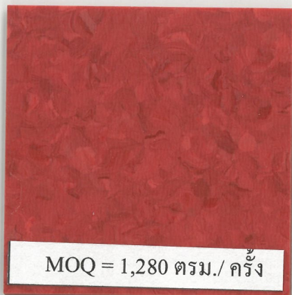
2612 Read
