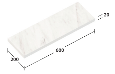
Code: WC-2060.2 200x600x20 mm. 8.33 pcs./sq.m. 6 pcs./ctn. 0.72 sq.m./ctn.
